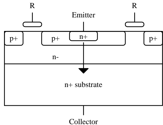
Fig. 8. Bipolar image sensor (BASIS) developed by Canon.
