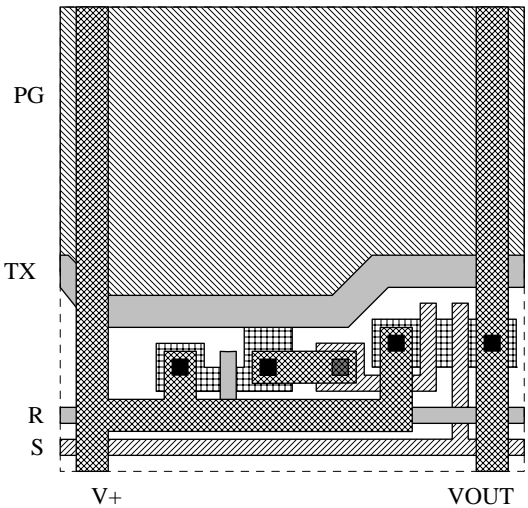
Fig. 3. Layout of a simple CMOS-compatible APS pixel.
